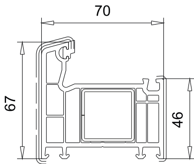
Frame art. 102.208
