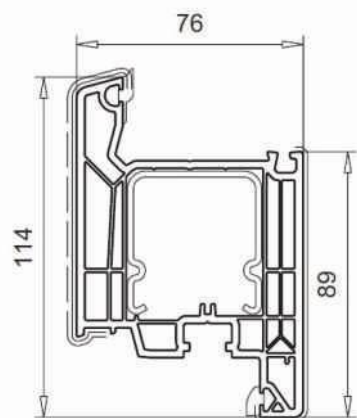
Sash art. 103.485
