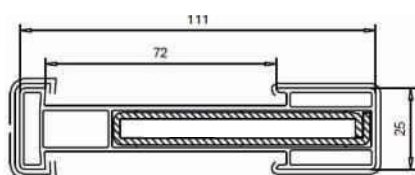
I-beam art. 116.228.2
