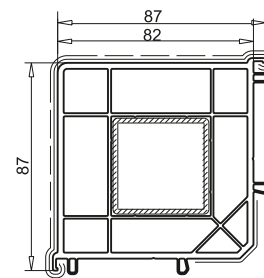
Square profile art. 116.229
