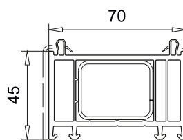
Expander art. 114.202
