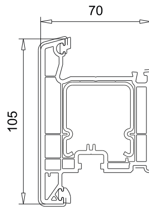
Sash art. 103.242
