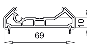
Corner connector adapter art. 116.205
