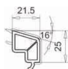
Glazing bead 32 mm art. 107.267
