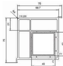
Square profile art. 116.200
