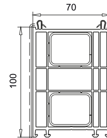
Expander art. 114.203
