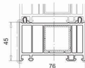
Expander art. 114.054
