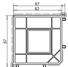
Square profile art. 116.229
