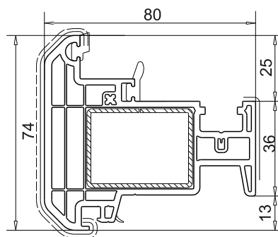
Stulp art. 102.316
