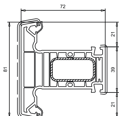
Mullion art. 102.346
