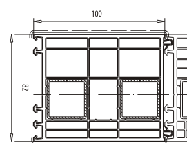
Expander art. 114.043
