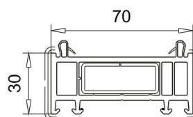
Expander art. 114.201
