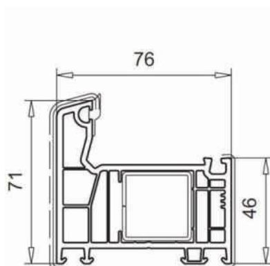
Frame art. 101.353
