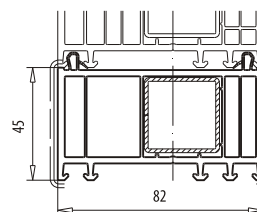
Expander art. 114.042
