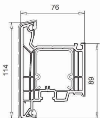
Sash art. 103.486
