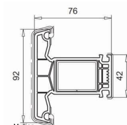
Mullion art. 102.352
