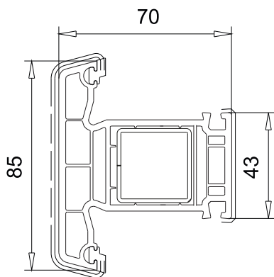
Mullion art. 102.214
