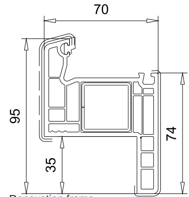
Renovation frame art. 101.218
