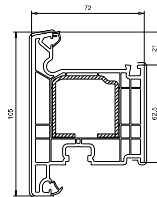
Sash art. 103.376
