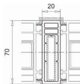
I-beam art. 116.201
