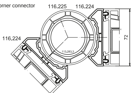
Corner connector
