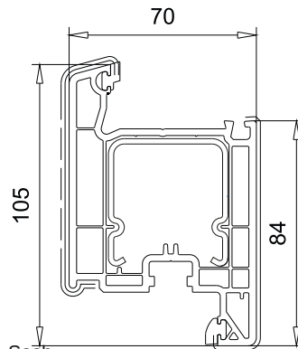
Sash art. 103.241
