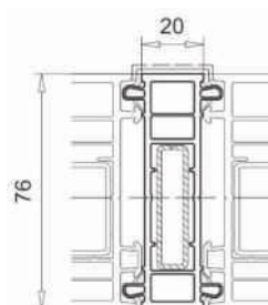
I-beam art. 116.230
