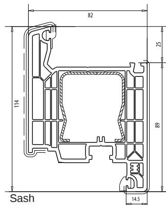
Sash art. 103.346
