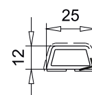
Applied muntin art. 109.587
