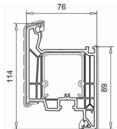
Sash art. 113.485
