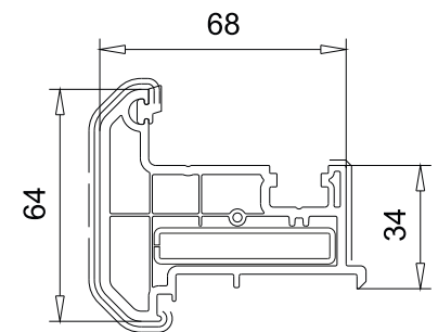
Stulp art. 102.236
