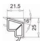
Glazing bead 32 mm art. 107.267
