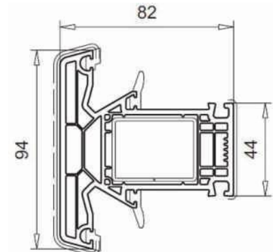
Mullion art. 102.310
