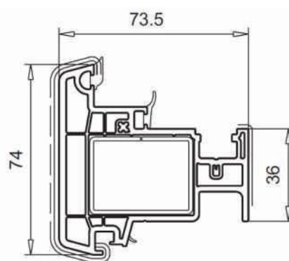
Stulp art. 102.356
