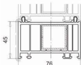
Expander art. 114.054
