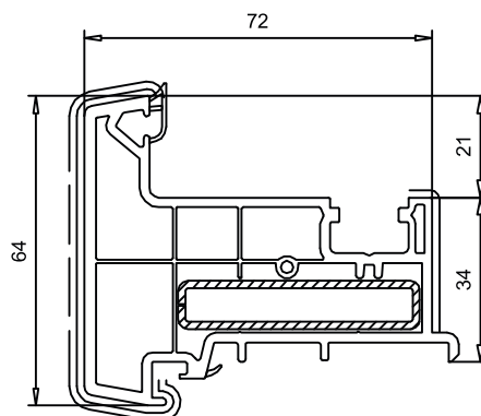
Stulp art. 102.340
