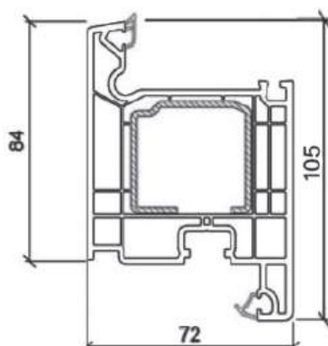
Sash art. 103.408
