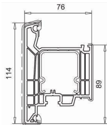
Sash art. 103.486
