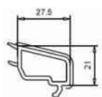
Glazing bead 24 mm art. 107.143
