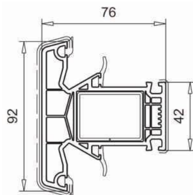
Mullion art. 102.350
