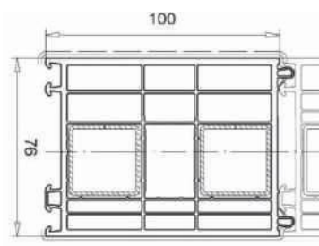
Expander art. 114.055
