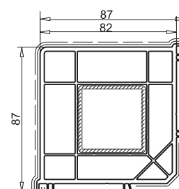
Square profile art. 116.229
