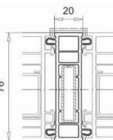
I-beam art. 116.230
