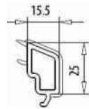
Glazing bead 44 mm art. 107.264
