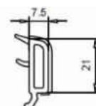
Glazing bead 44 mm art. 107.228
