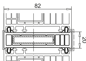
I-beam art. 116.219
