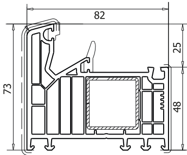
Frame art. 101.290
