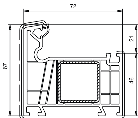
Frame art. 101.310
