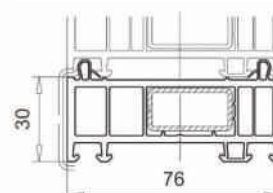
Expander art. 114.053
