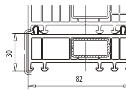
Expander art. 114.041
