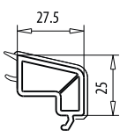
Glazing bead 32 mm art. 107.269
