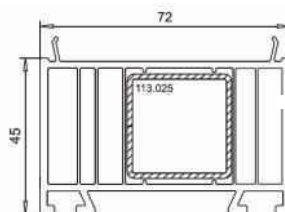
Expander art. 113.025
