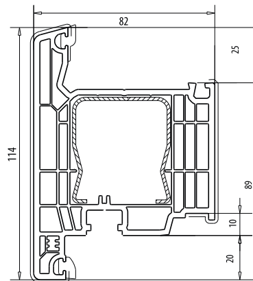
Sash art. 103.346
