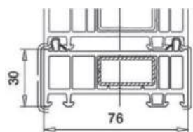
Expander art. 114.053
