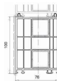
Expander art. 114.055
