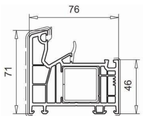
Frame art. 101.350
